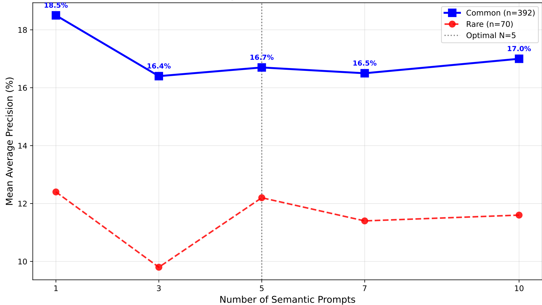
Effect of Prompt Count on AP — Saturation at N=5
